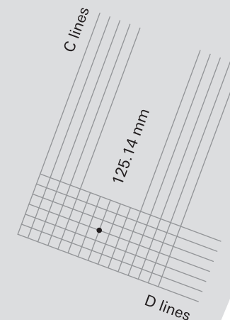
Stylus point of AT-FTT for zero tracking error
